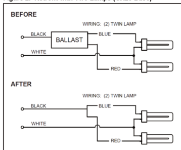
Figure 2. Retrofit with Two Lamps (GX23 Base)
