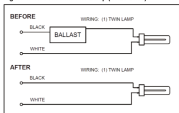
Figure 1. Retrofit with One Lamp (GX23 Base)
