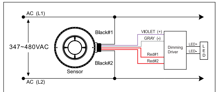
Wiring with dimming ballast or LED driver. Dimming Sensor
