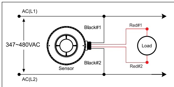
Wiring with non-dimming ballast or LED driver. ON/OFF Sensor
