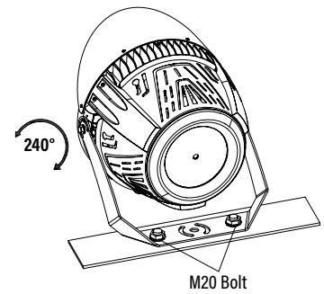
INSTALL METHOD 2
