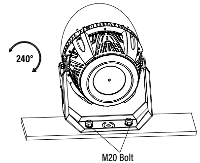
INSTALL METHOD 2
