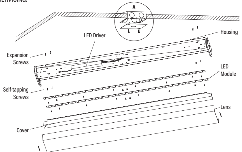
A - Concealed Outlet Box
