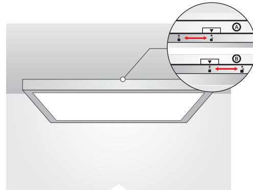
STEP 3: Align the bracket to final position (angle). Mount 4 dry wall plugs (provided) in ceiling through the bracket.
