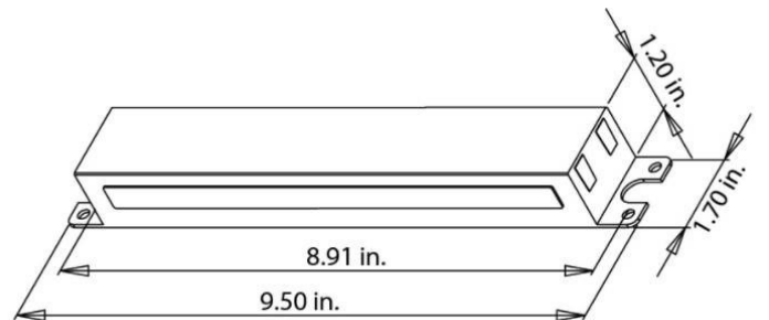
4 Channel Driver
