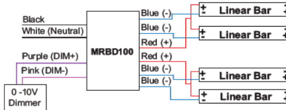
Four-bar configuration
