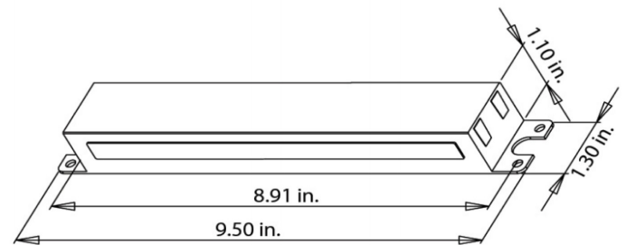
2 Channel Driver
