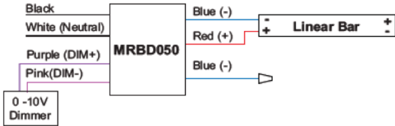
One-bar configuration
