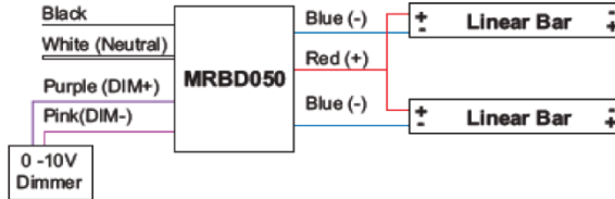
Two-bar configuration
