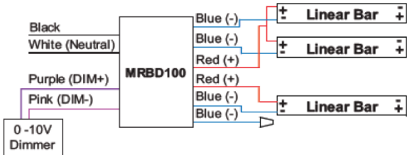
Three-bar configuration
