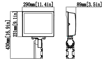
105-140W Slipfitter Knuckle (CCT Selectable)
