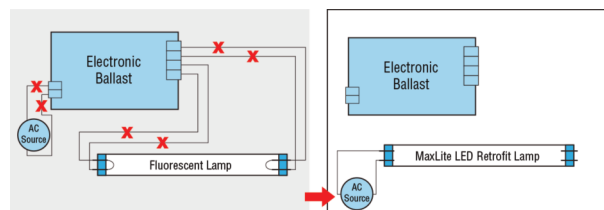
Figure 3. - Retrofit with One Lamp
