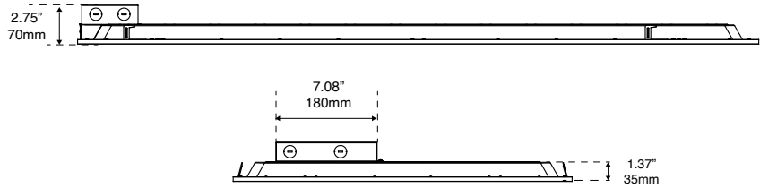
WITH J-BOX
