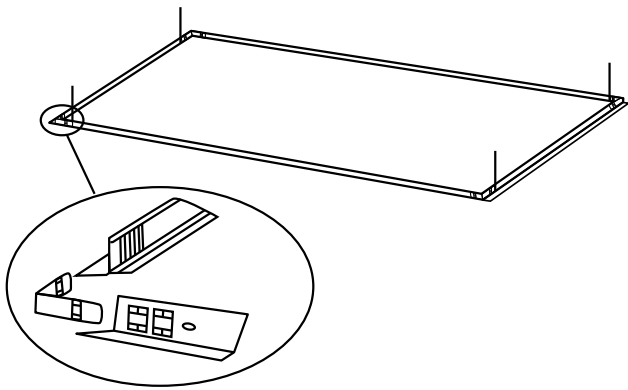
2x4 Flange Kit Ceiling opening is 24.25" x 48.25"
