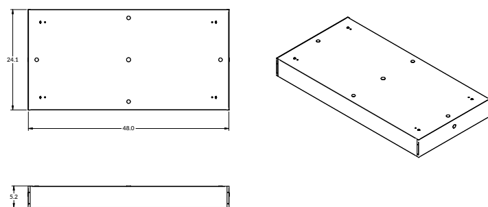
2x4 w/ SM Surface Mount Kit
