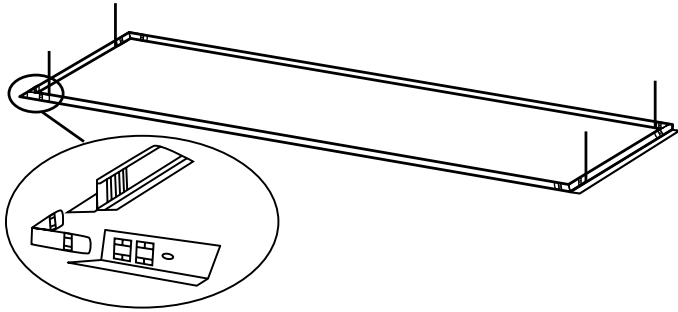
1x4 Flange Kit Ceiling opening is 12.25" x 48.25"
