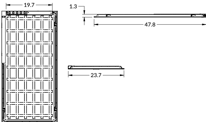
2x4 VPAN-CR-EM8
