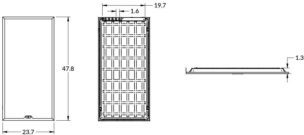
2x4 VPAN-CR
