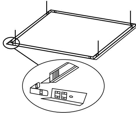
2x2 Flange Kit Ceiling opening is 24.25" x 24.25"
