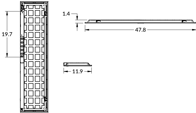
1x4 VPAN-EM8
