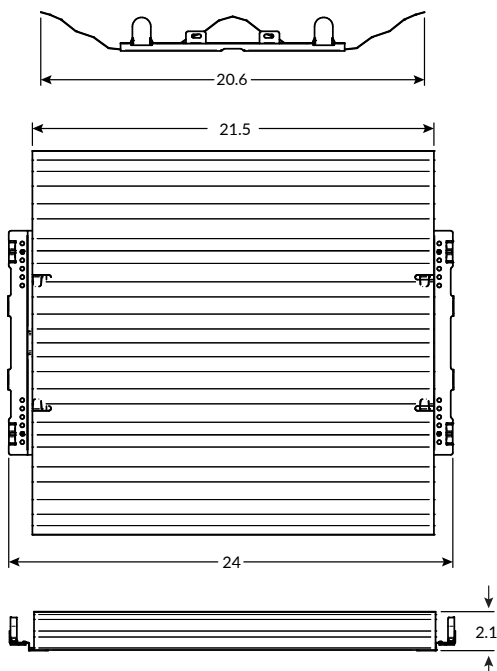
2x2 Configuration
