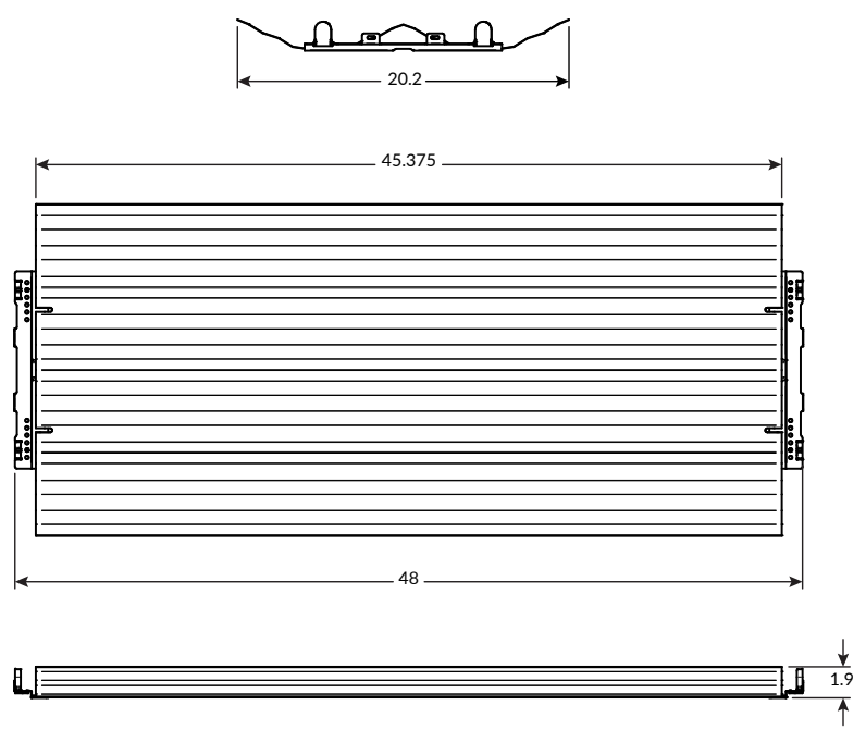
2x4 Configuration
