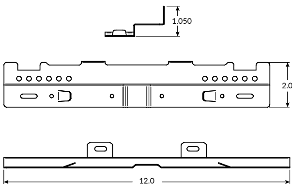
2 Lamp Configuration
