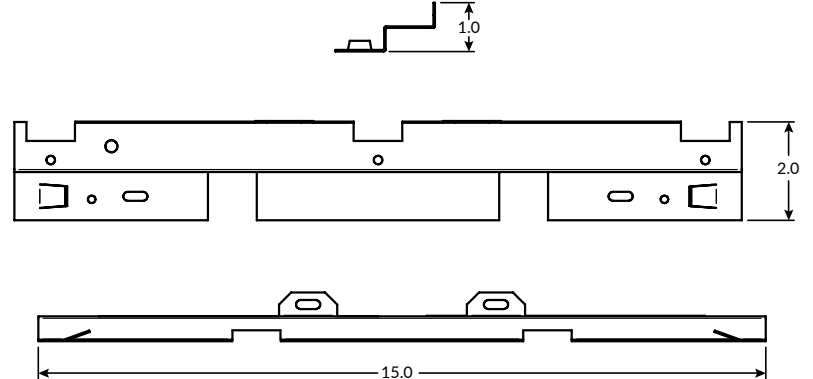
3 Lamp Configuration
