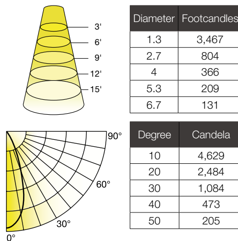
24PAR38HODIM/9CCTS/277V/SD - 40°
