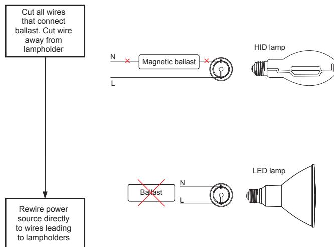
Diagram 4 – Magnetic ballast fixture wiring modification
