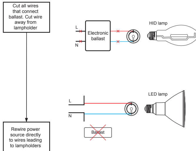
Diagram 3 – Electronic ballast fixture wiring modification
