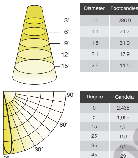
7.5MR16DIM/927SP10/RC + MR/ACC/LN1225
