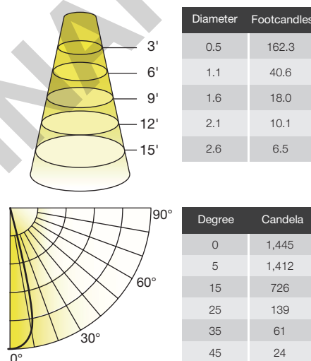
7.5MR16DIM/927SP10/RC + MR/ACC/SQ2525
