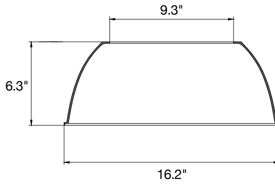
Acrylic Reflector (90°) RHB-100/150-ACR-RF
