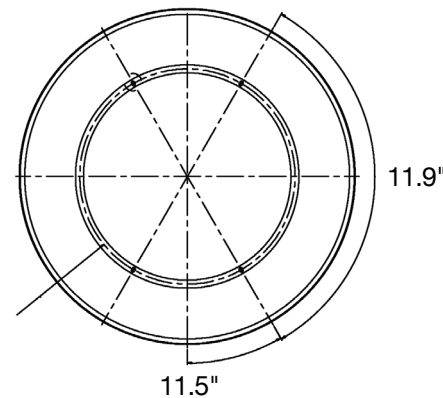
Wire Guard RHB3-240-WG
