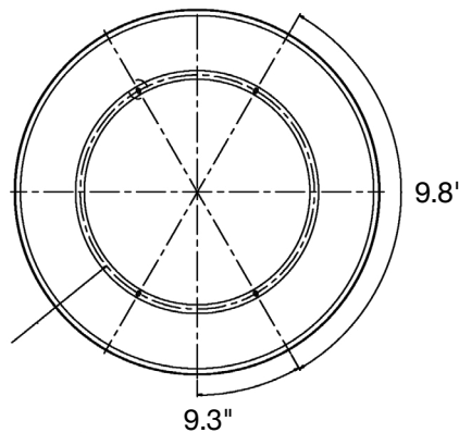
Wire Guard RHB3-100/150-WG
