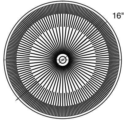
Acrylic Bottom Cover (90°) RHB-UNV-ACR-BC
