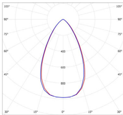
60° x 60° Medium Beam (MB) Directional floodlight for general lighting
