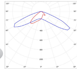
50° x 140° Type II (2) Wide-walkways, roadway entrances, and mass access points. (Intended for pole or wall mounting)
