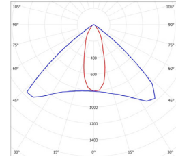
30° x 100° Type I (1) Paths, walkways and sidewalks (Intended for center area mounting)
