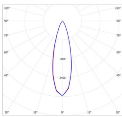
30° x 30° Narrow Beam (NB) Spotlight or concentrated applications
