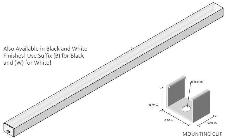
MOUNTING CLIP
