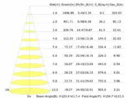
Illuminance at a Distance (Beam Angle)
